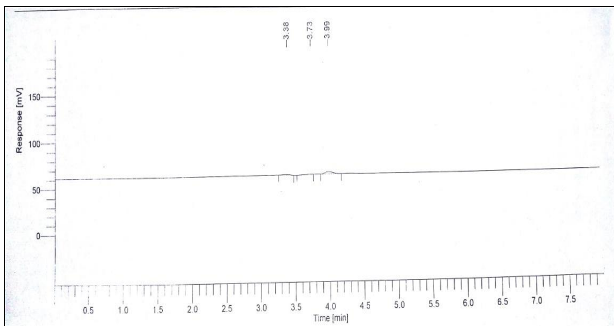
Fig. 4: Chromatogram of Placebo solution
