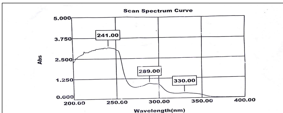
Fig. 2: UV Spectra of Lenvatinib
