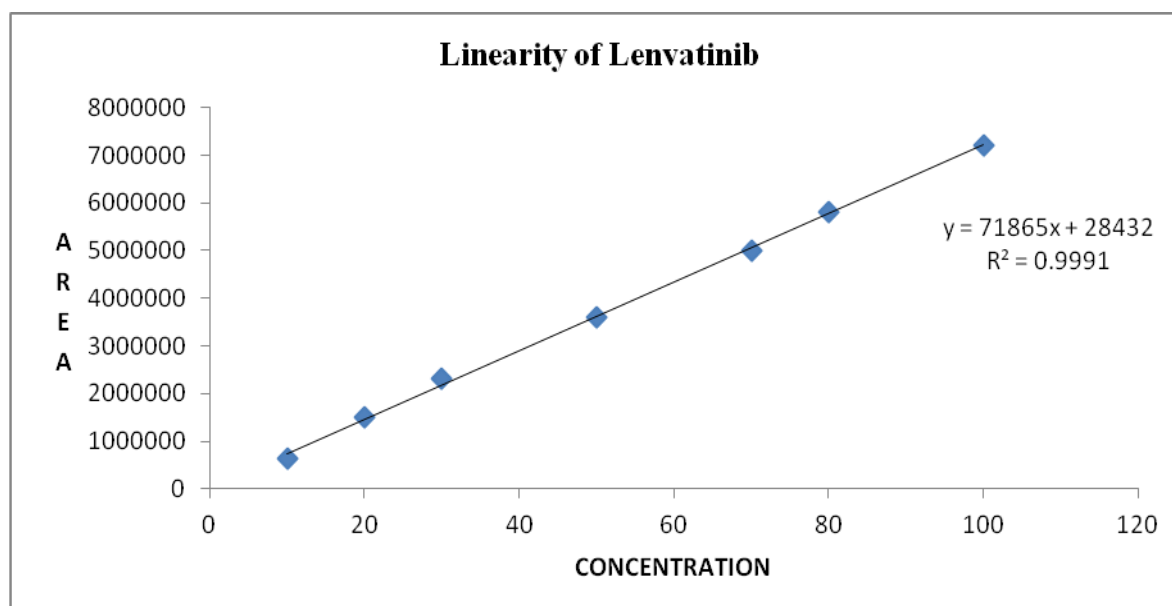
Fig. 7: Linearity Plot of Lenvatinib
