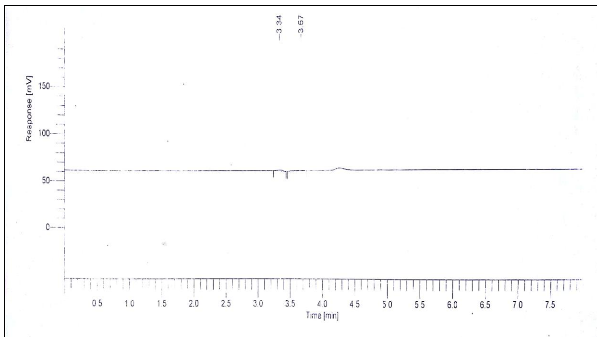
Fig. 3: Chromatogram of Blank solution
