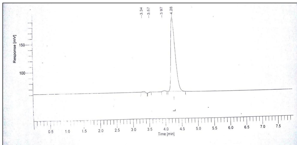
Fig. 6: Chromatogram of Lenvatinib sample solution
