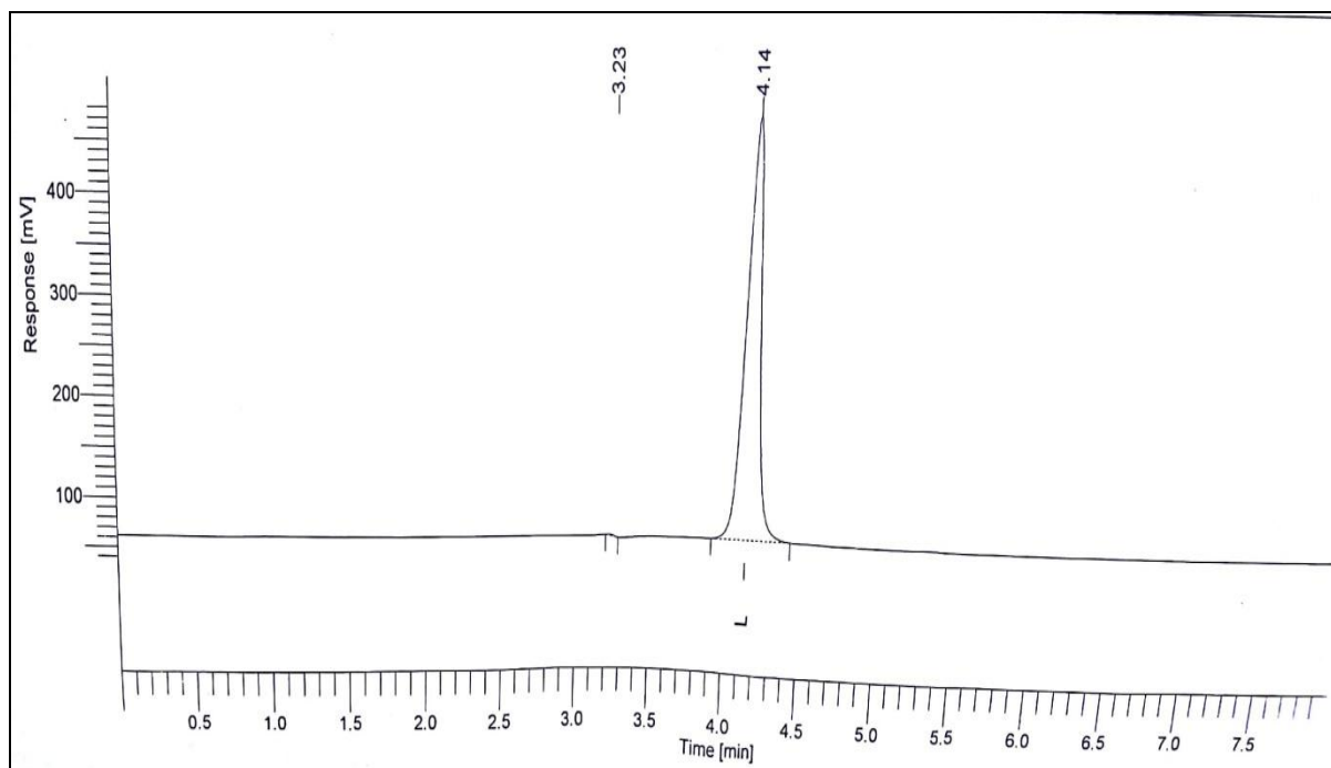
Fig. 5: Chromatogram of Lenvatinib standard solution
